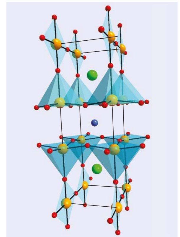
Fig. 3. Atomic structure of one of the best-known high-temperature superconductors, \text{YBa}_2\text{Cu}_3\text{O}_7 , showing the position of copper (orange), oxygen (red), barium (green) and yttrium (blue) atoms. The material is highly anisotropic and pairing occurs in the \text{CuO}_2 planes. By removing oxygen far from the planes, one can change the average number of conduction electrons.
