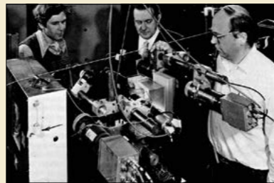
Tests on proton radiography using a beam from the 200 MeV booster at Argonne and a brain specimen in a water-filled box.
