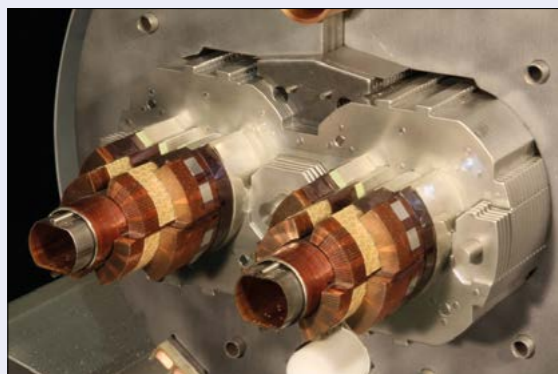
Industry-manufactured coils for an LHC main dipole carrying the two beam pipes, which guide protons on their circular path.
