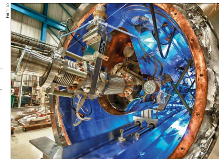
A superconducting RF capture cavity at Fermilab.
