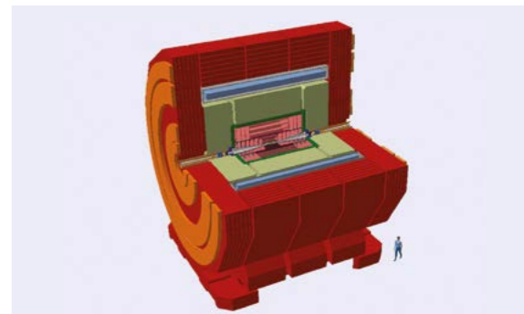
A detector magnet design under consideration for a future 100 TeV proton-proton collider (top image), measuring roughly 18 m in diameter and 49 m long, as part of the CERN co-ordinated Future Circular Collider project. The single-detector concept for CLIC (lower image), which measures roughly 12 m long and 13 m high.
