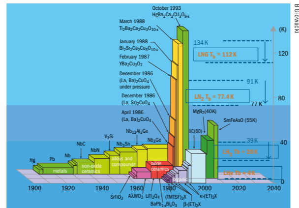
Fig. 2. Materials with record superconducting transition temperatures as a function of time, showing BCS superconductors, iron-based superconductors and high-temperature cuprate superconductors. The current record holder is a BCS-type superconductor, hydrogen sulphide, under a gigantic pressure of 155 GPa (not shown).
