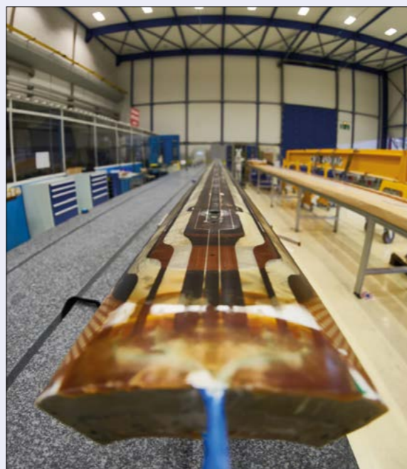
New long coils for the \text{Nb}_3\text{Sn} quadrupoles for the HL-LHC.
