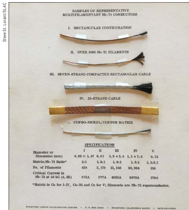
A selection of niobium-titanium wires in various configurations. Today, competition in the MRI market has driven down the cost of this particular superconductor.
