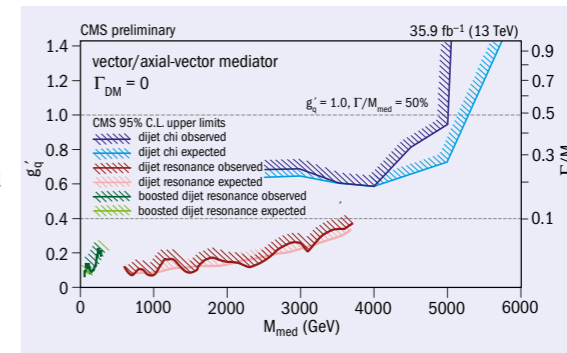
Top: 95% C.L. upper limits on the universal quark coupling g'_q (left vertical axis), and the resonance decay width \Gamma divided by mass (right vertical axis) as a function of the mass of the mediator (a leptophobic resonance). Bottom: Feynman diagrams showing the production of a new particle and its decay to quarks (left), with a gluon radiated from the initial state (middle) and a t-channel diagram governing the QCD dijet background (right).
