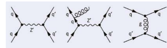
Top: 95% C.L. upper limits on the universal quark coupling g'_q (left vertical axis), and the resonance decay width \Gamma divided by mass (right vertical axis) as a function of the mass of the mediator (a leptophobic resonance). Bottom: Feynman diagrams showing the production of a new particle and its decay to quarks (left), with a gluon radiated from the initial state (middle) and a t-channel diagram governing the QCD dijet background (right).
