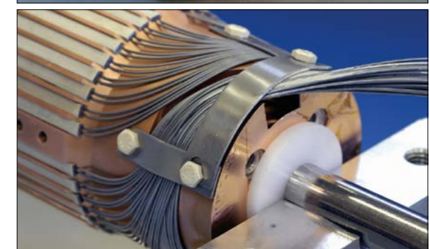
Fig. 3. When cooled to 1.9 K, the LHC's niobium-titanium cables can conduct the same current as a bundle of copper wires 11 cm high and 8 cm wide (top). The cables are made from 36 strands with a diameter of 0.825 mm, each of which comprises 6500 superconducting filaments of niobium-titanium surrounded by a 0.0005 mm layer of high-purity copper. (Above) A close-up of the lower part of a 13 kA high-temperature superconducting current lead for powering the LHC main dipole magnets, which contains the material BSCCO-2223. The technology, the first application of HTS materials in a large-scale accelerator system, allows the room-temperature power cables from the power converters to be connected to the cold Nb-Ti bus-bars of the LHC magnets.
