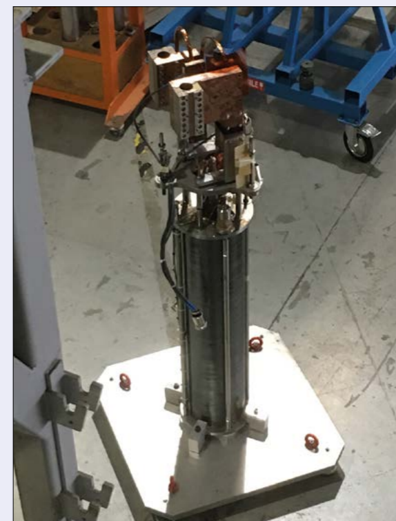
The Feather2 HTS demonstration magnet pictured in CERN’s SM18 facility in July.
