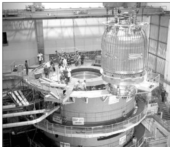
In the early 1970s, CERN's Big European Bubble Chamber, now an exhibit at the lab, was equipped with the largest superconducting magnet in service at the time.
