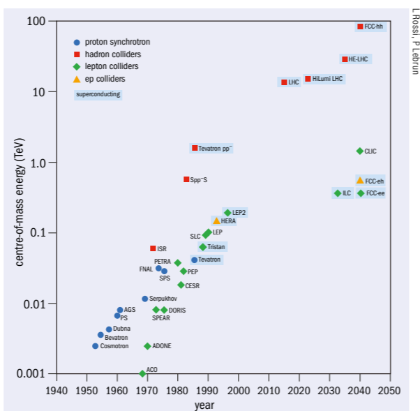
Fig. 1. Particle energy (in the centre-of-mass reference frame) as a function of time, showing various types of collider and the proposed parameters for new colliders at the energy frontier. Since the Tevatron (1983), through HERA (1991), RHIC (2000) and finally the LHC (2008), all large-scale hadron colliders have been built using superconducting magnets.
