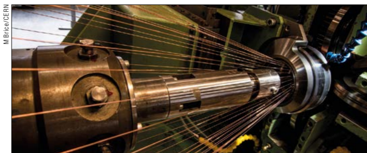
Cable for the High-Luminosity LHC magnets being produced at CERN.
