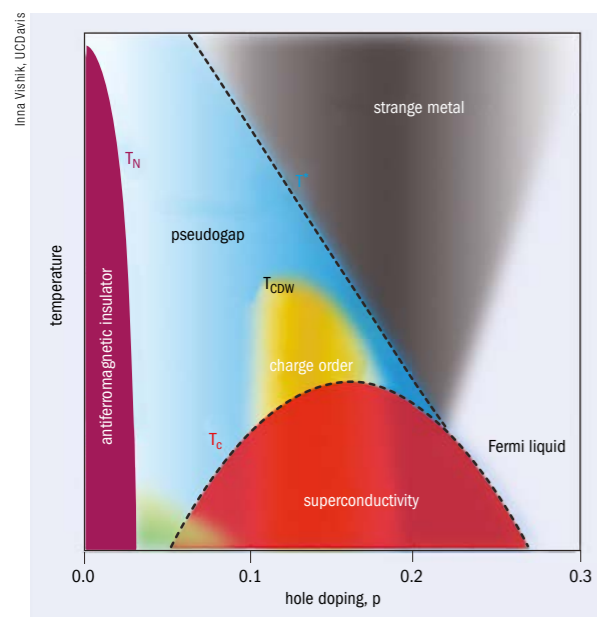
Fig. 4. The phase diagram of a typical cuprate superconductor. When plotted as a function of temperature and hole-doping, p (where p = 0 means one conduction electron per copper atom), many different phases appear: the most prominent are antiferromagnetism near p = 0 and a superconductivity dome at larger doping. In the “pseudogap” region, states disappear at low energy, while above this line the metallic state is different from an ordinary metal and is called a strange metal.
