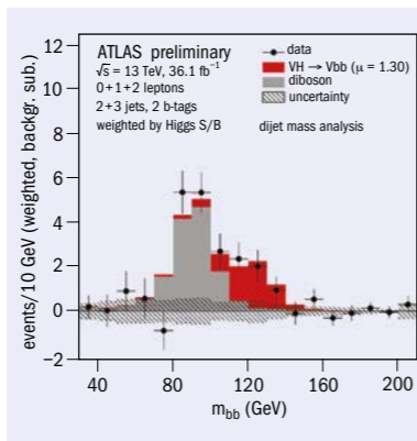
Mass distribution of the two-b-jet system after subtraction of all backgrounds except for those arising from VZ and Z \rightarrow bb . The contribution of the Higgs boson is shown in red and the contribution of VZ in grey, the observation of which provides a powerful validation of the analysis.
