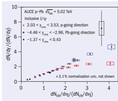
The J/ψ yield relative to the measurement in minimum-bias collisions in three rapidity regions, as a function of relative charged-particle multiplicity measured at central pseudorapidity.
