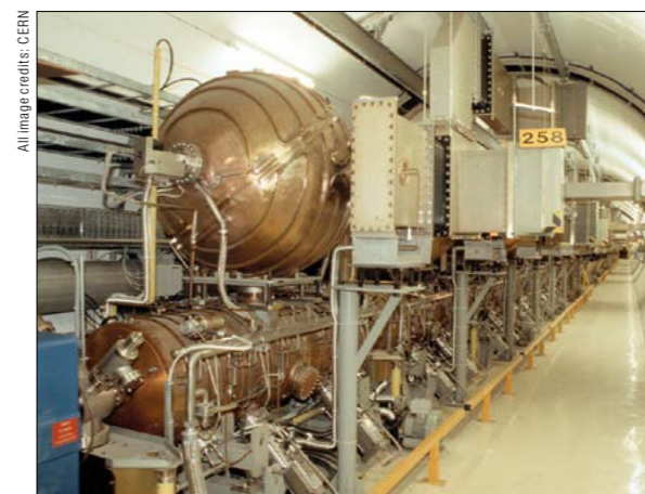
The copper cavities used to accelerate particles in LEP (above). Replacement superconducting RF cavities installed in the LEP tunnel (above right) and their niobium accelerating structures (bottom right) allowed the collider's energy to be doubled in the late 1990s, beyond the pair-production threshold for W bosons.
